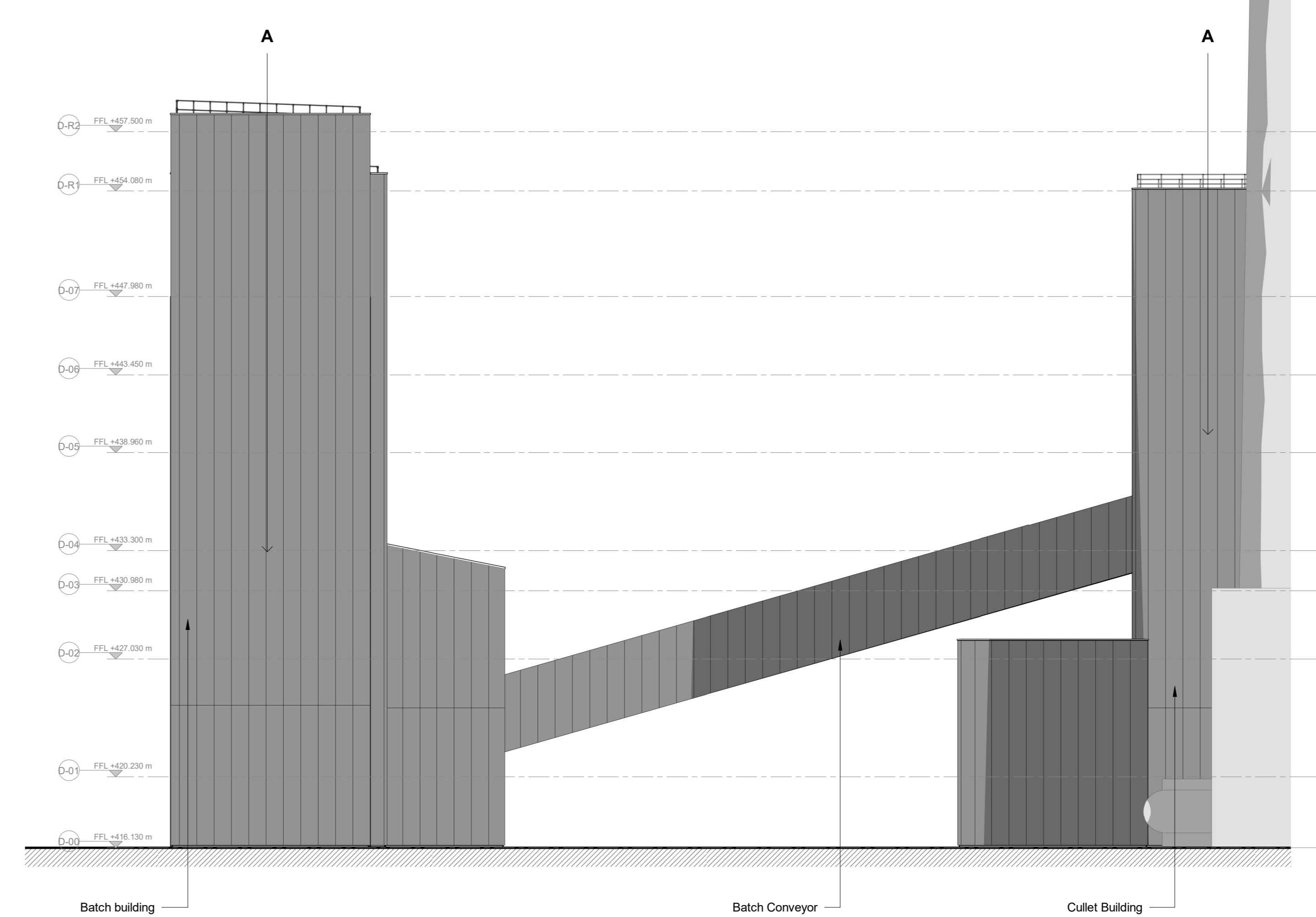
2 Elevation Batch - South (Planning) 1: 200
