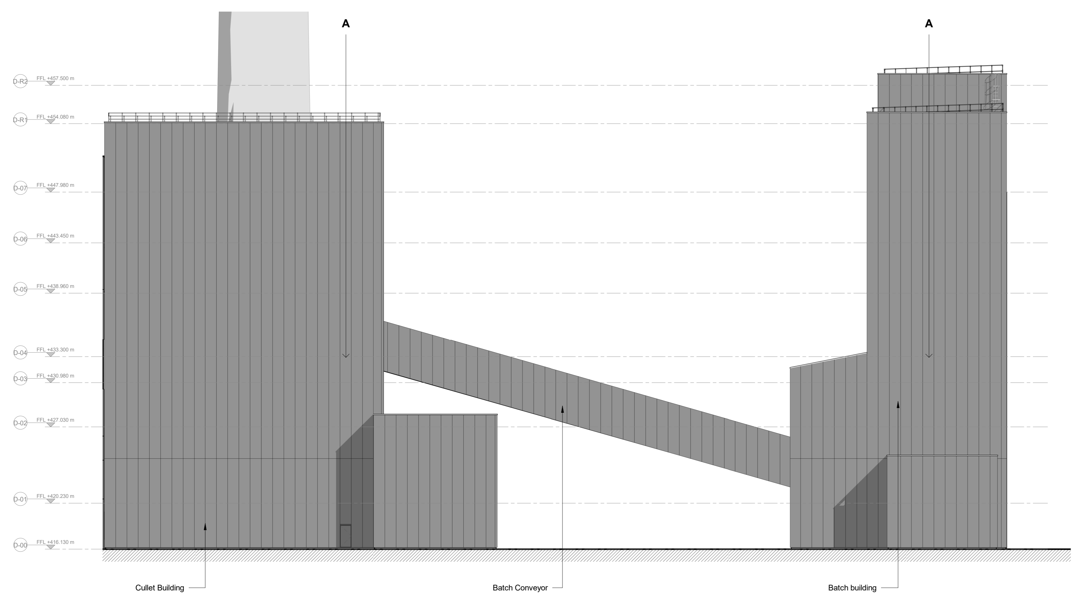
1 Elevation Batch - North (Planning) 1: 200
